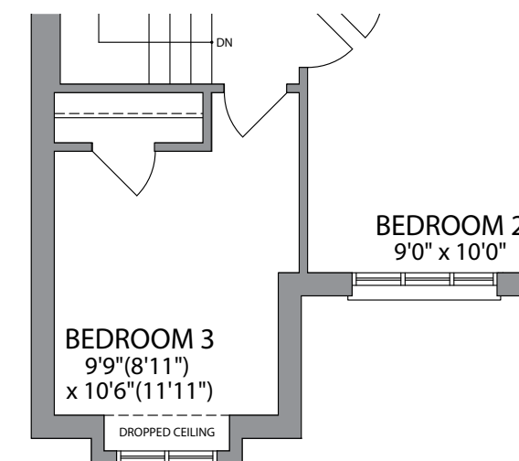
OPT. SECOND FLOOR W/4 BEDROOMS ELEVATION 2A (4A SIMILAR)
