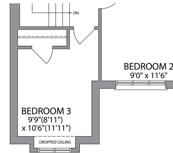
SECOND FLOOR ELEVATION 2A (4A SIMILAR)
