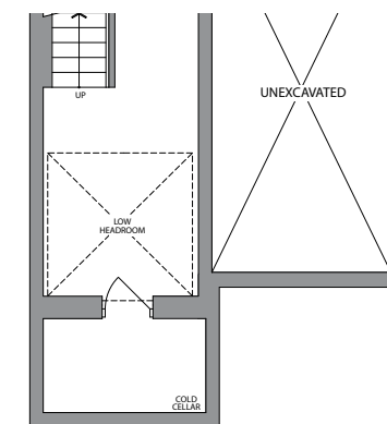
BASEMENT ELEVATION 3 & 4
