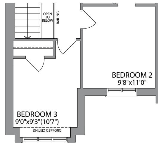
SECOND FLOOR ELEVATION 2
