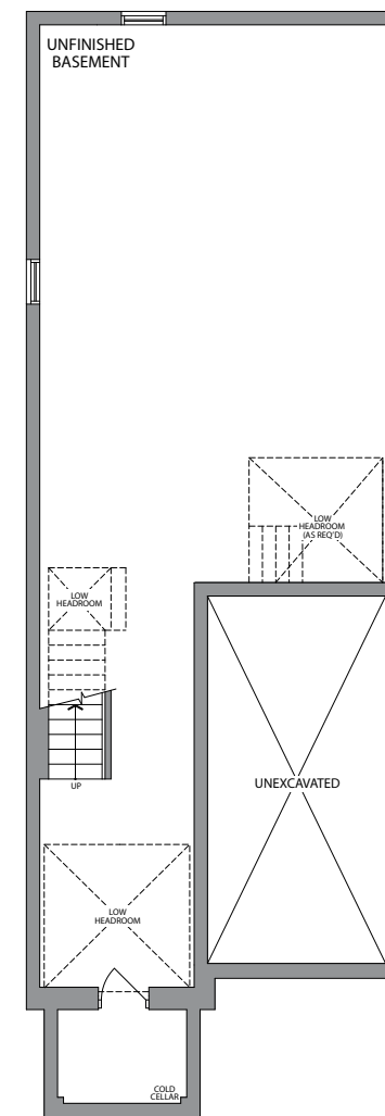
BASEMENT ELEVATION 1 & 2
