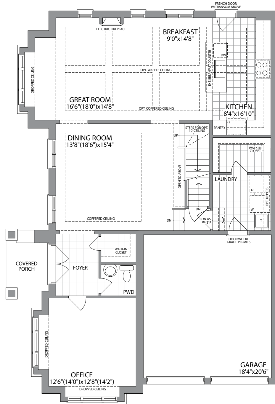
GROUND FLOOR ELEVATION 1C
