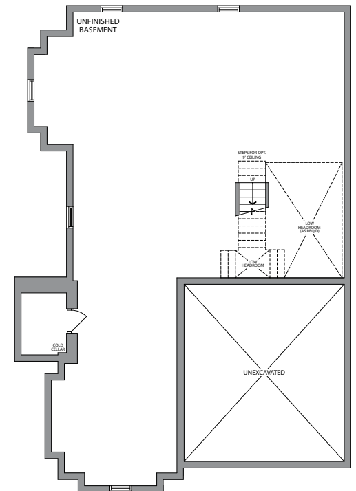
BASEMENT ELEVATION 1C
