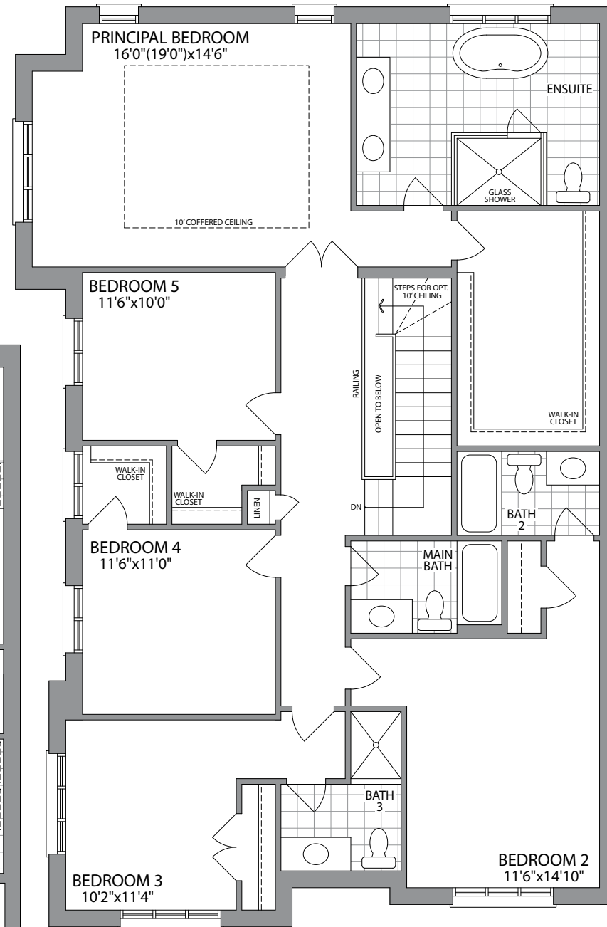
SECOND FLOOR ELEVATION 1C
