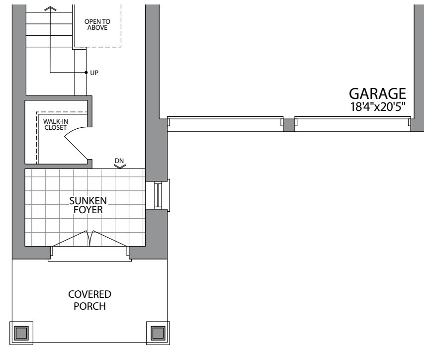
GROUND FLOOR ELEVATION 3
