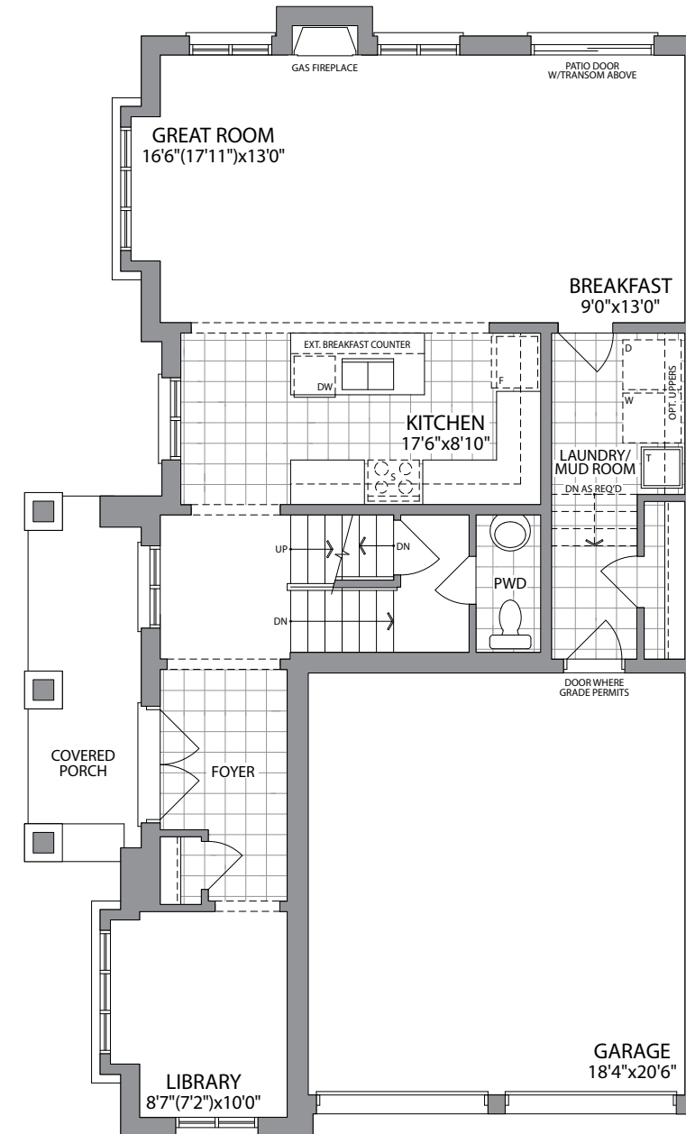
GROUND FLOOR ELEVATION 3C
