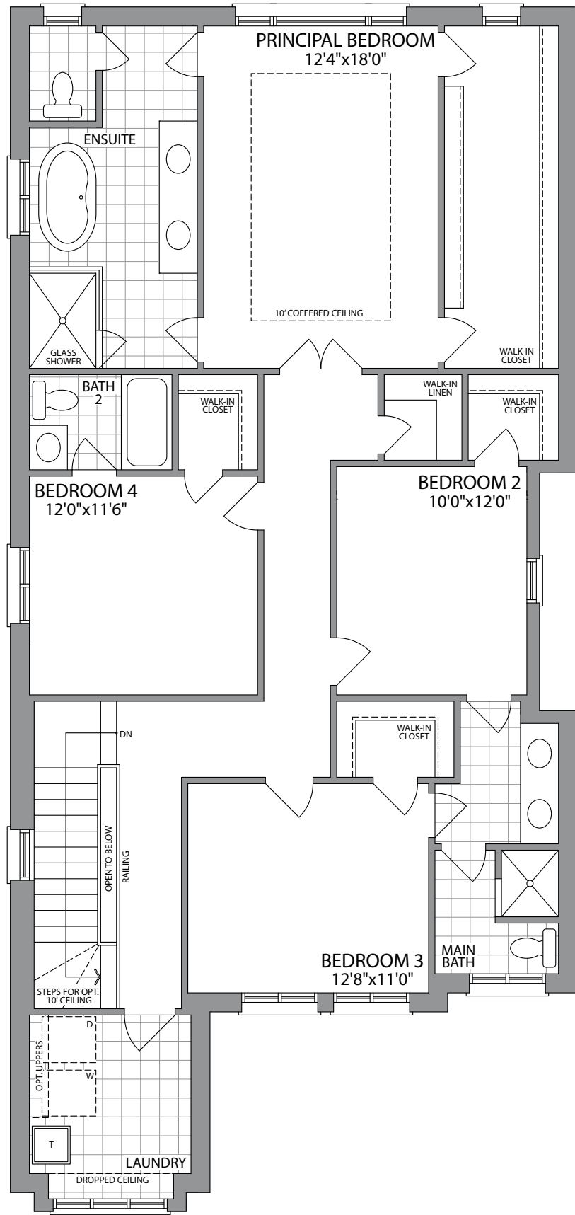
SECOND FLOOR ELEVATION 1
