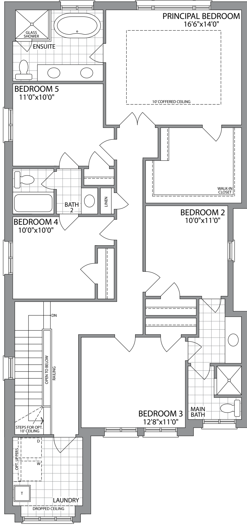
OPT. SECOND FLOOR W/5 BEDROOMS ELEVATION 1
