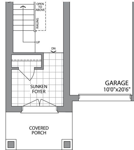
GROUND FLOOR ELEVATION 3 & 4
