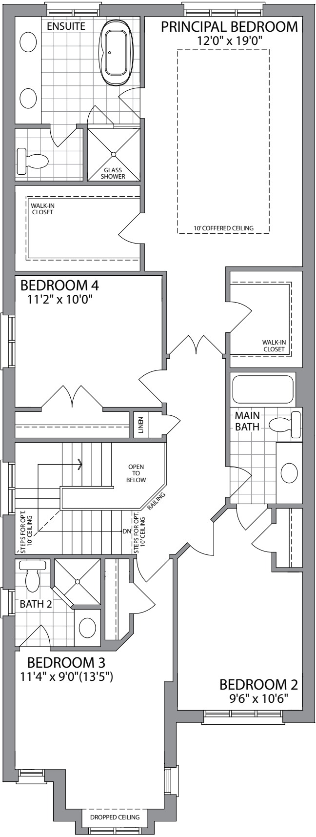
SECOND FLOOR ELEVATION 3
