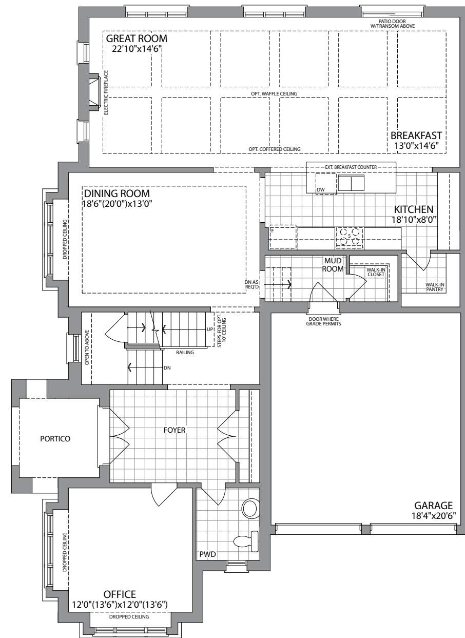
GROUND FLOOR ELEVATION 1C
