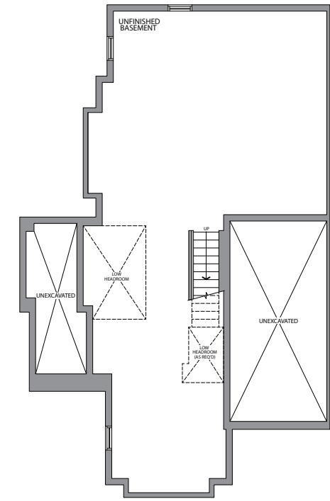
BASEMENT ELEVATION 3C
