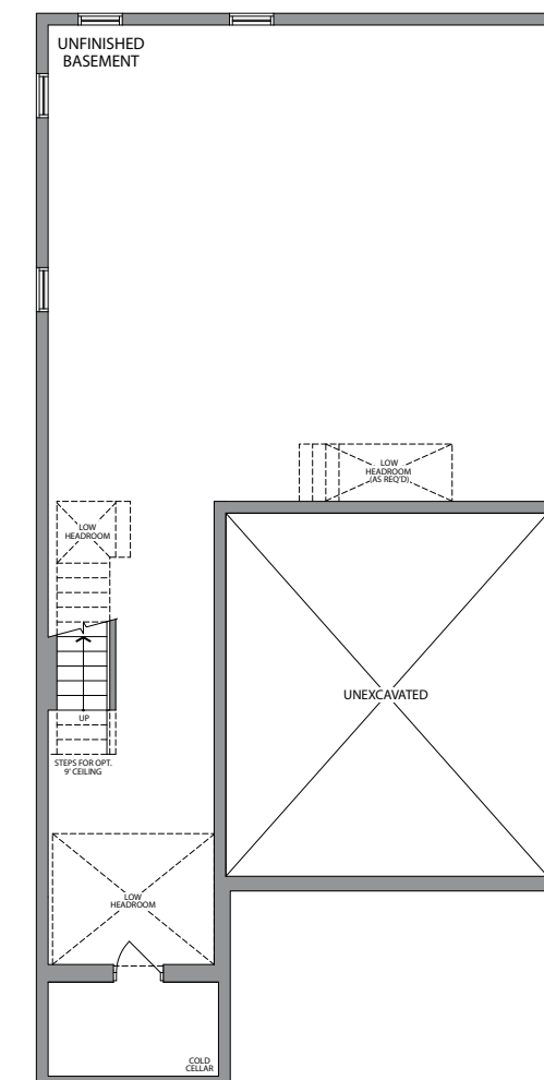
BASEMENT ELEVATION 1
