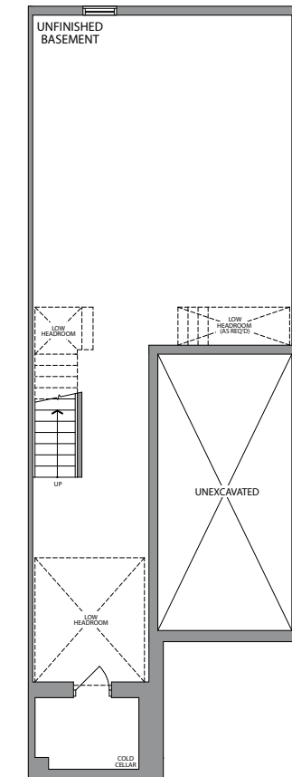
BASEMENT ELEVATION 1
