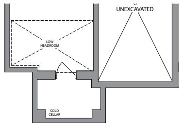
BASEMENT ELEVATION 2
