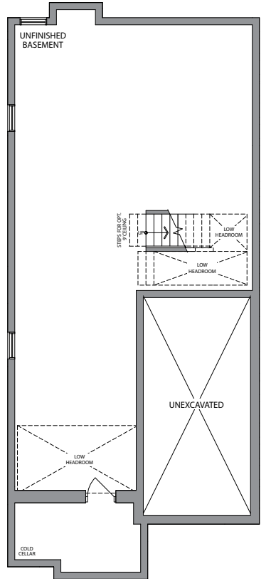
BASEMENT ELEVATION 3
