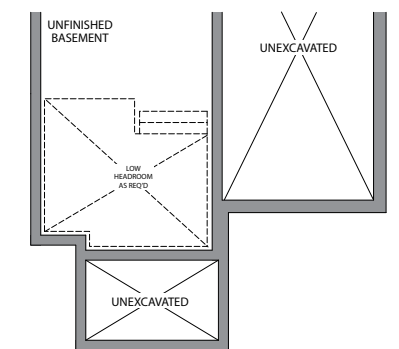
BASEMENT ELEVATION 2
