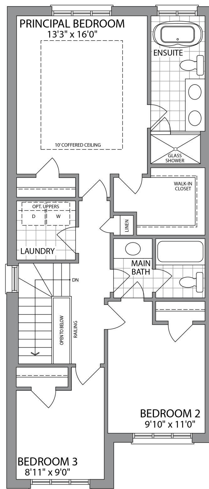
SECOND FLOOR ELEVATION 1
