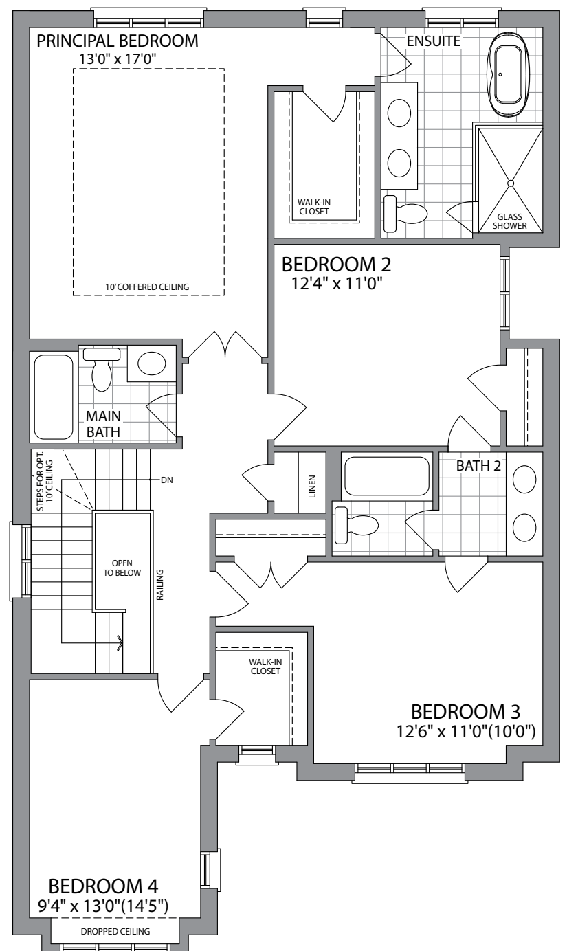
SECOND FLOOR ELEVATION 3
