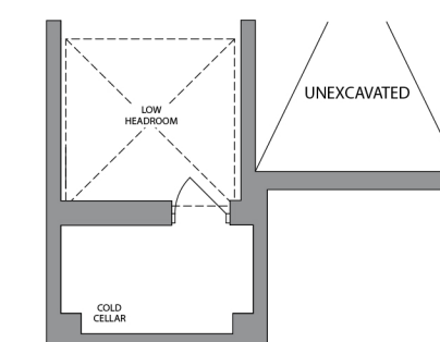
BASEMENT ELEVATION 3 & 4
