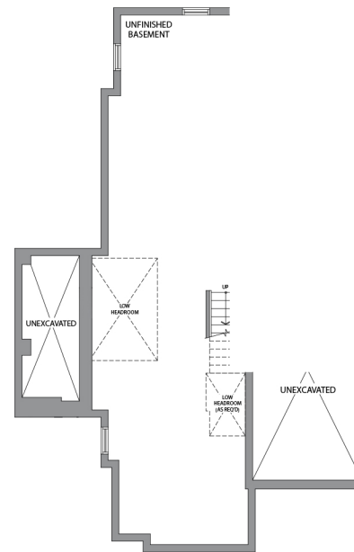
BASEMENT ELEVATION 2C
