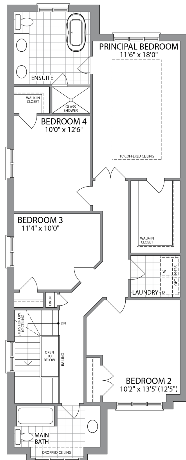
SECOND FLOOR ELEVATION 3
