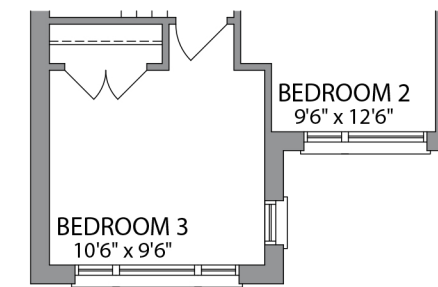
SECOND FLOOR ELEVATION 2C
