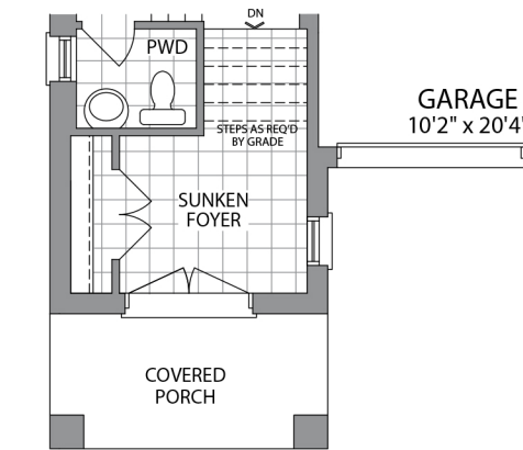
GROUND FLOOR ELEVATION 2C
