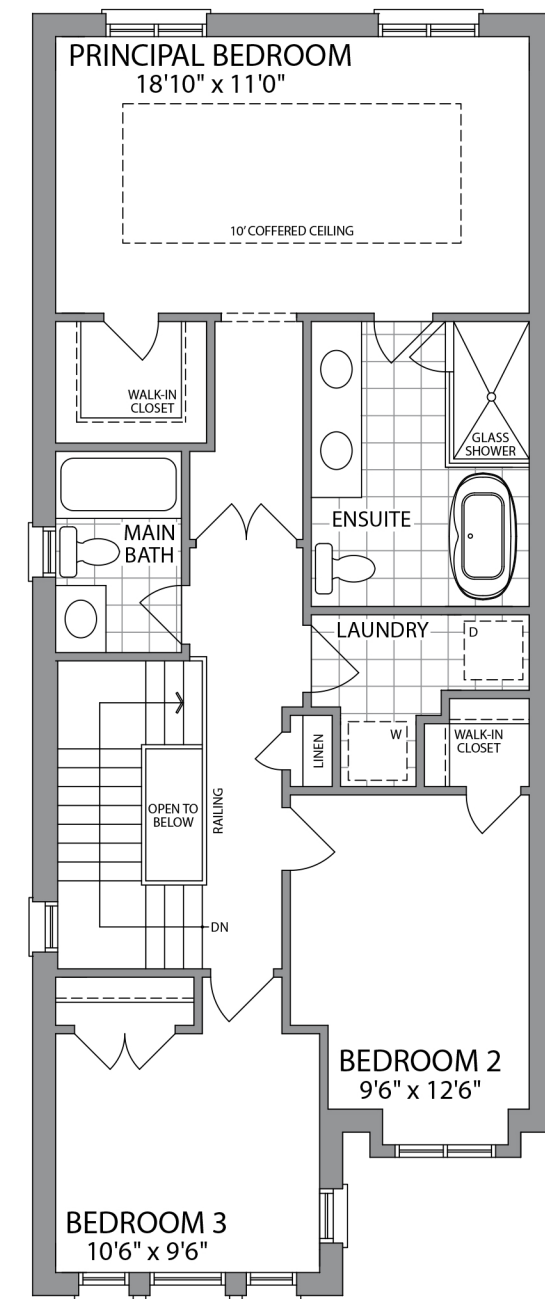
SECOND FLOOR ELEVATION 3C
