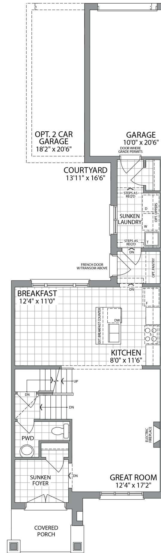
GROUND FLOOR ELEVATION 1
