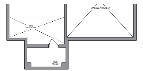
BASEMENT ELEVATION 2
