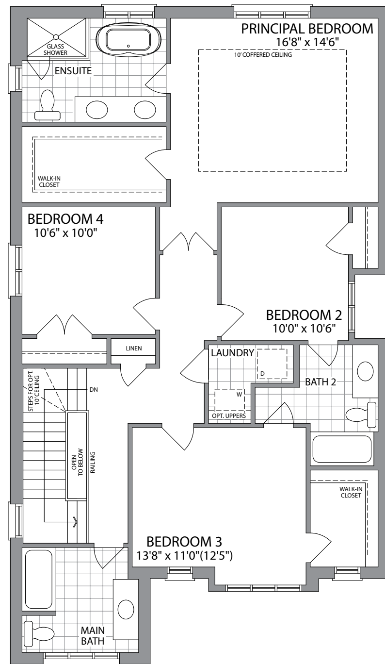
SECOND FLOOR ELEVATION 3
