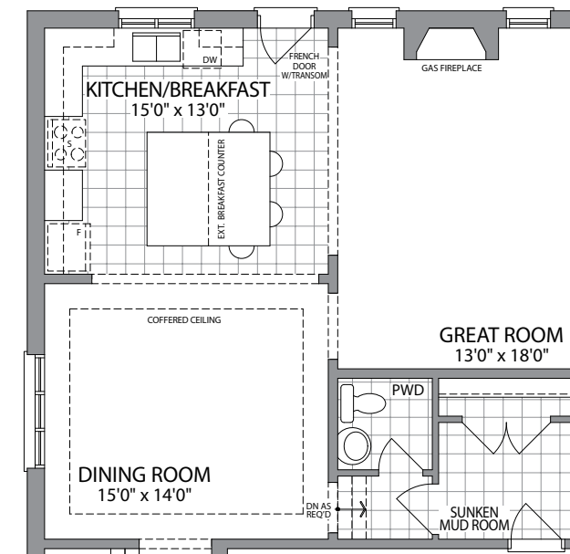
OPT. GROUND FLOOR
