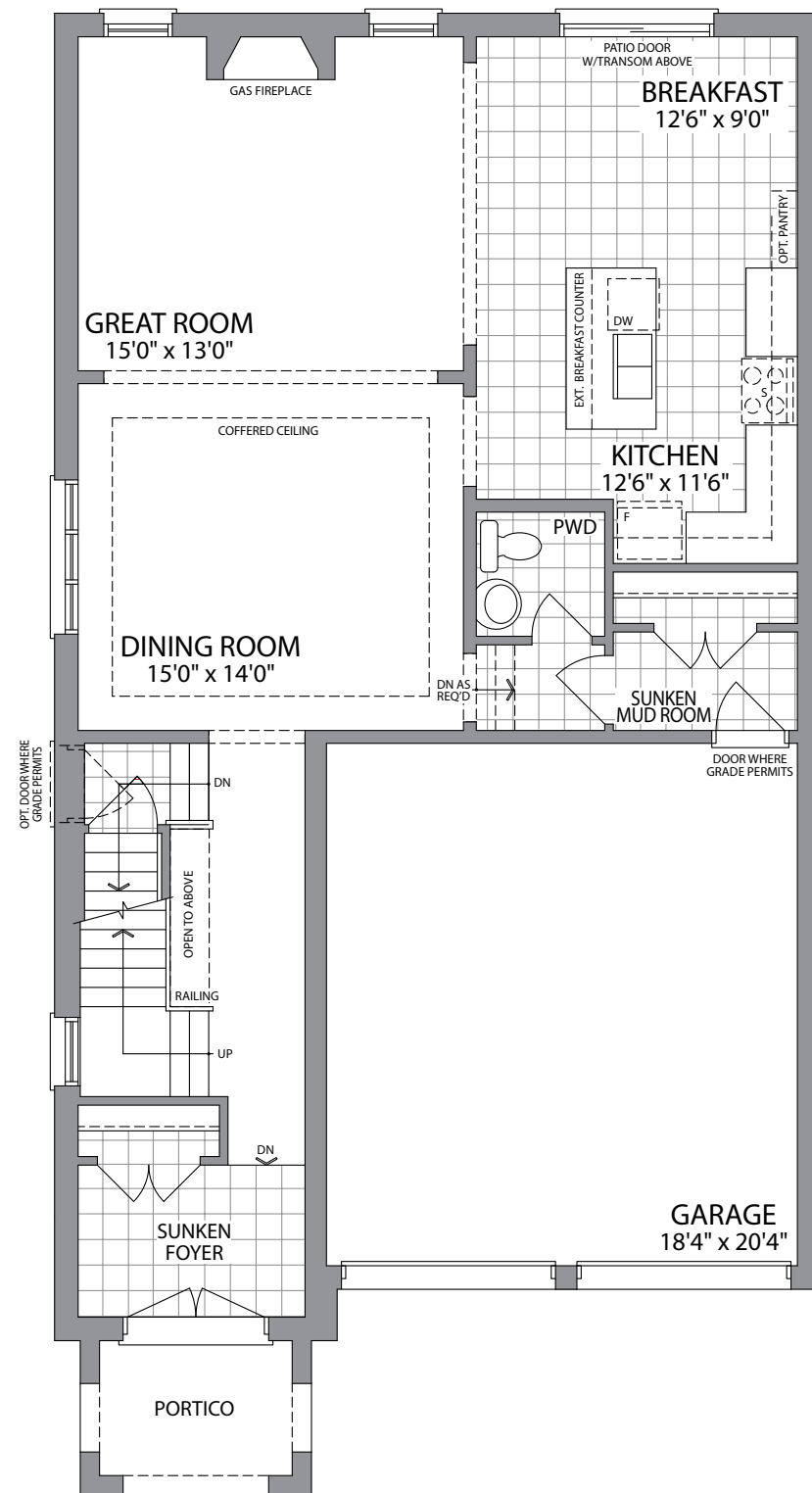
GROUND FLOOR ELEVATION 3
