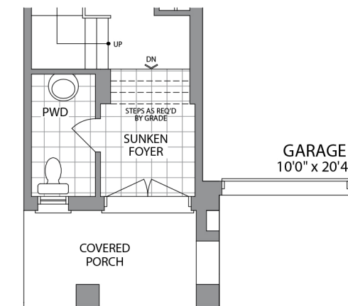
GROUND FLOOR ELEVATION 2
