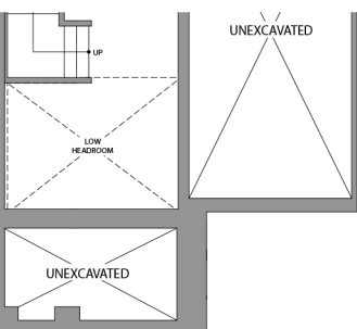
BASEMENT ELEVATION 2
