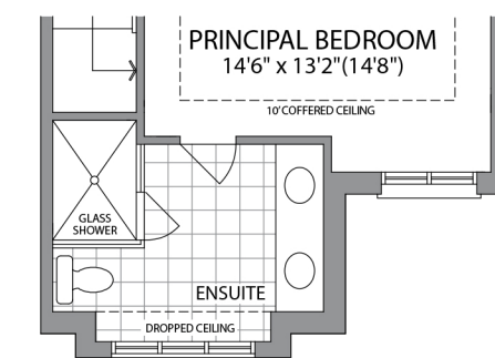
SECOND FLOOR ELEVATION 2
