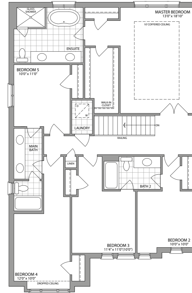
OPT. SECOND FLOOR W/5 BEDROOMS ELEVATION 1
