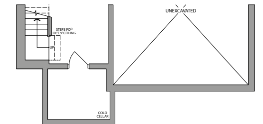
BASEMENT ELEVATION 2
