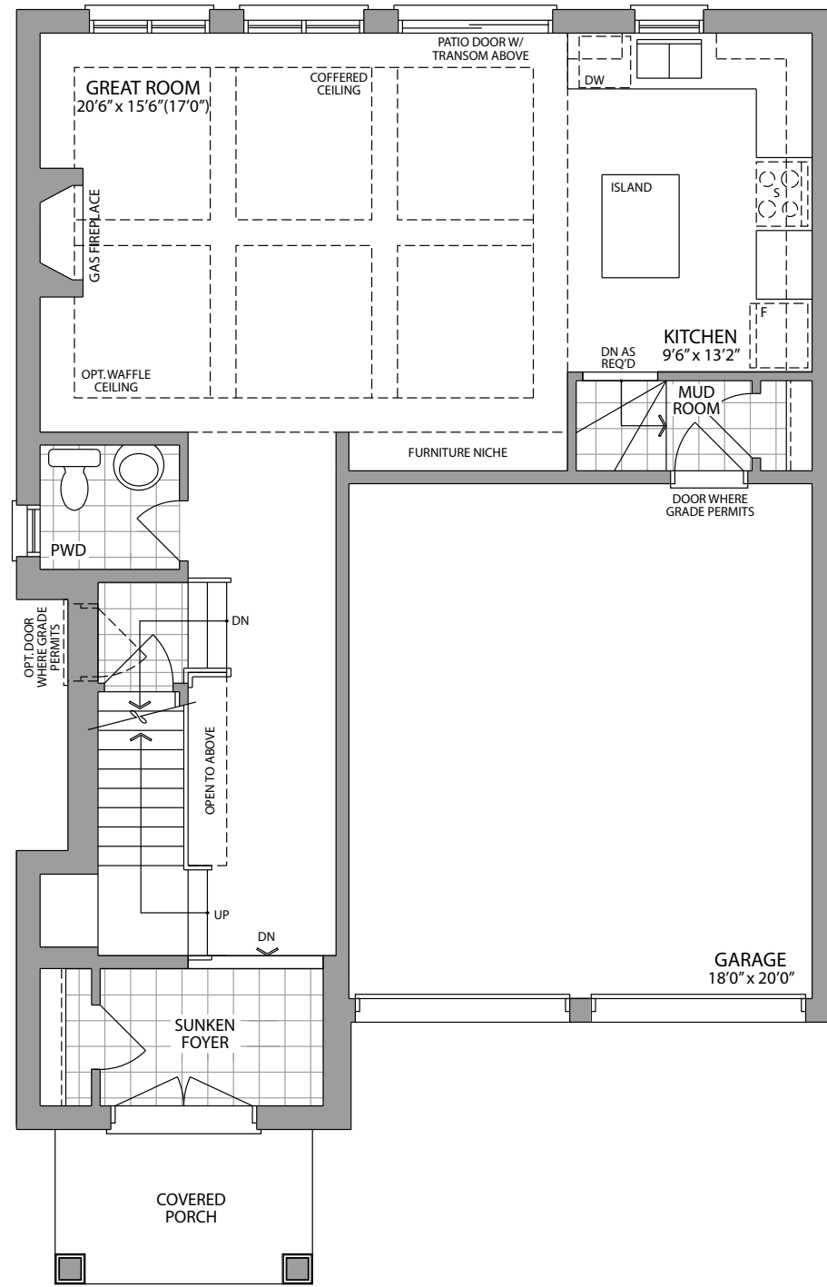
GROUND FLOOR ELEVATION 1
