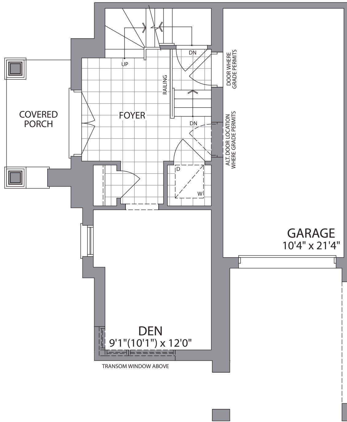
GROUND FLOOR ELEVATION 1C
