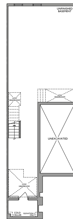
BASEMENT ELEVATION 1 & 2
