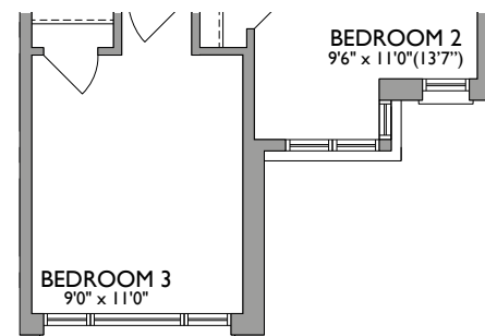
OPT. SECOND FLOOR 4 BEDROOM ELEVATION 2
