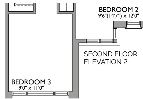
OPT. SECOND FLOOR 4 BEDROOM ELEVATION 2
