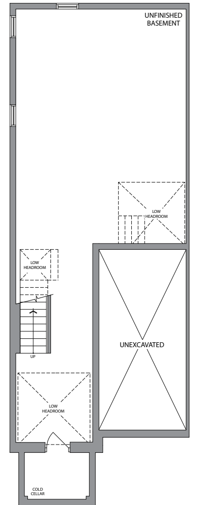
BASEMENT ELEVATION 1 & 2
