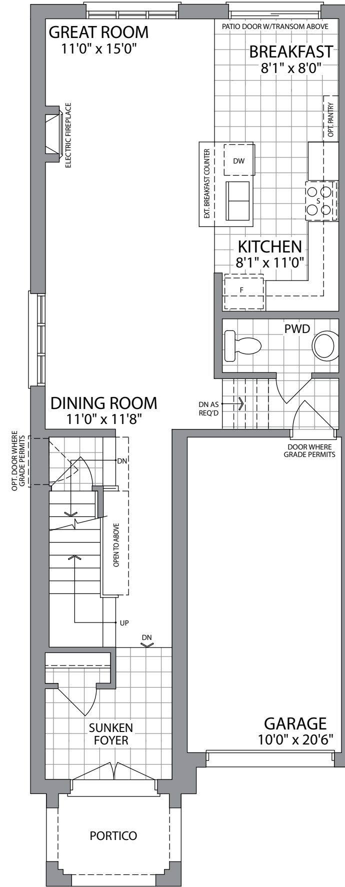
GROUND FLOOR ELEVATION 1 & 2
