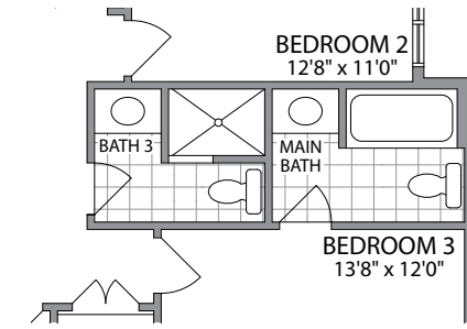
OPT. SECOND FLOOR W/EXTRA BATH ELEVATION 2C & 3C
