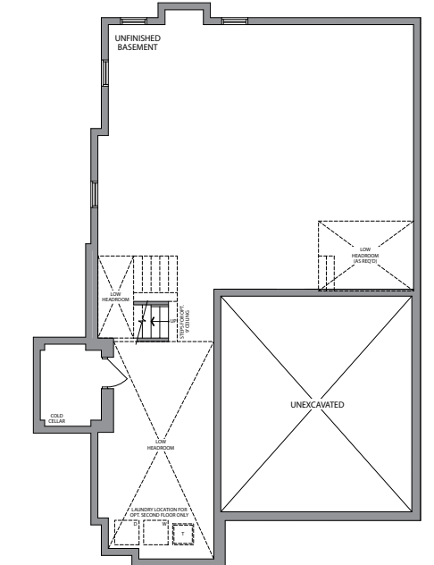
BASEMENT ELEVATION 2C
