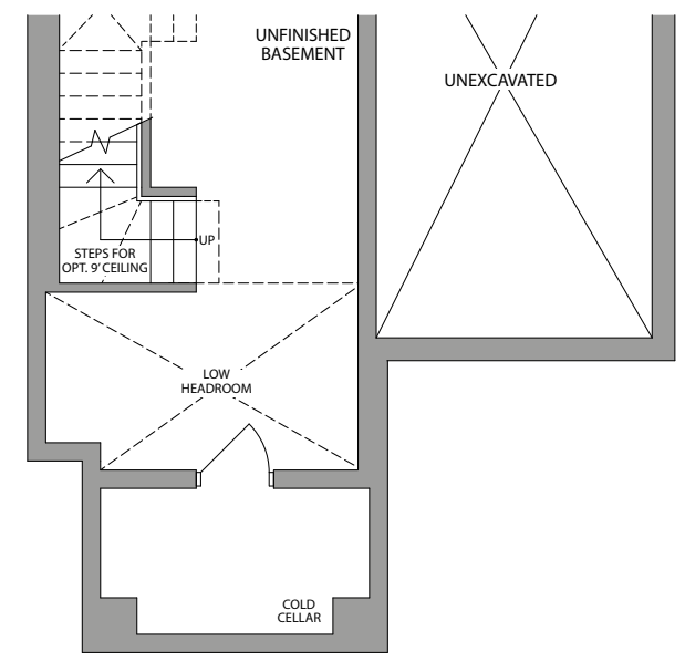
BASEMENT ELEVATION 2
