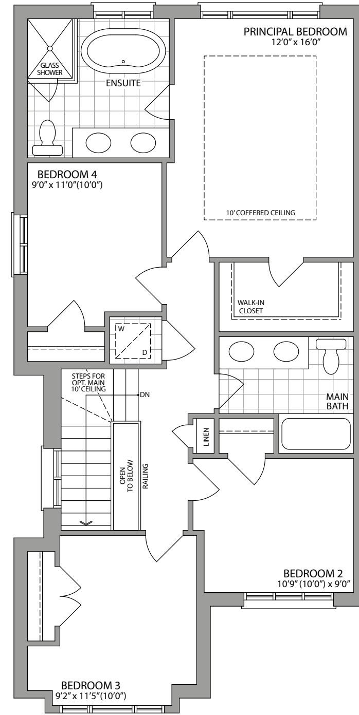
OPT. SECOND FLOOR W/4 BEDROOMS ELEVATION 1
