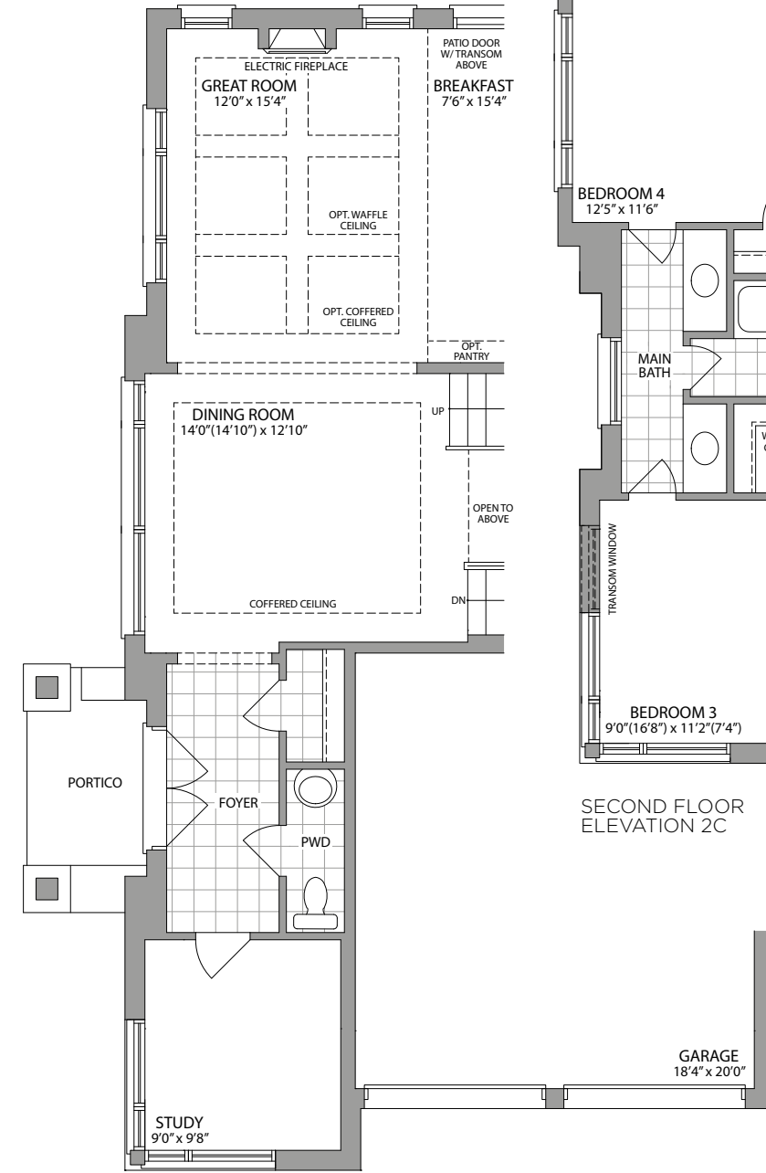
GROUND FLOOR ELEVATION 2C
