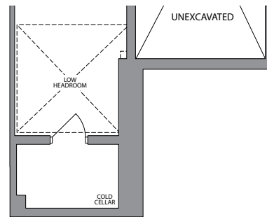
BASEMENT ELEVATION 2
