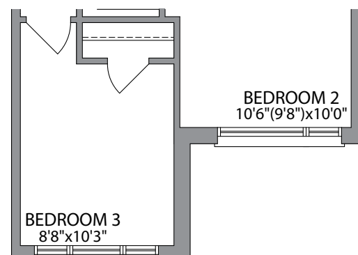
OPT. SECOND FLOOR W/4 BEDROOMS ELEVATION 3
