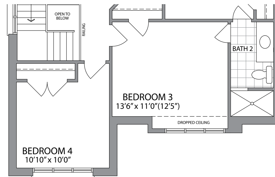
Second Floor Elevation 2
