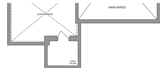
Basement Elevation 2
