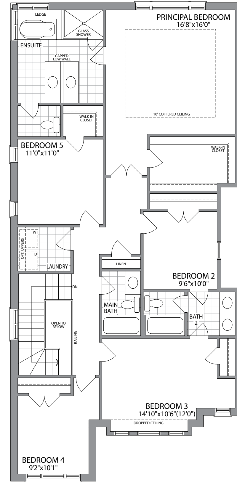
Second Floor Elevation 2
