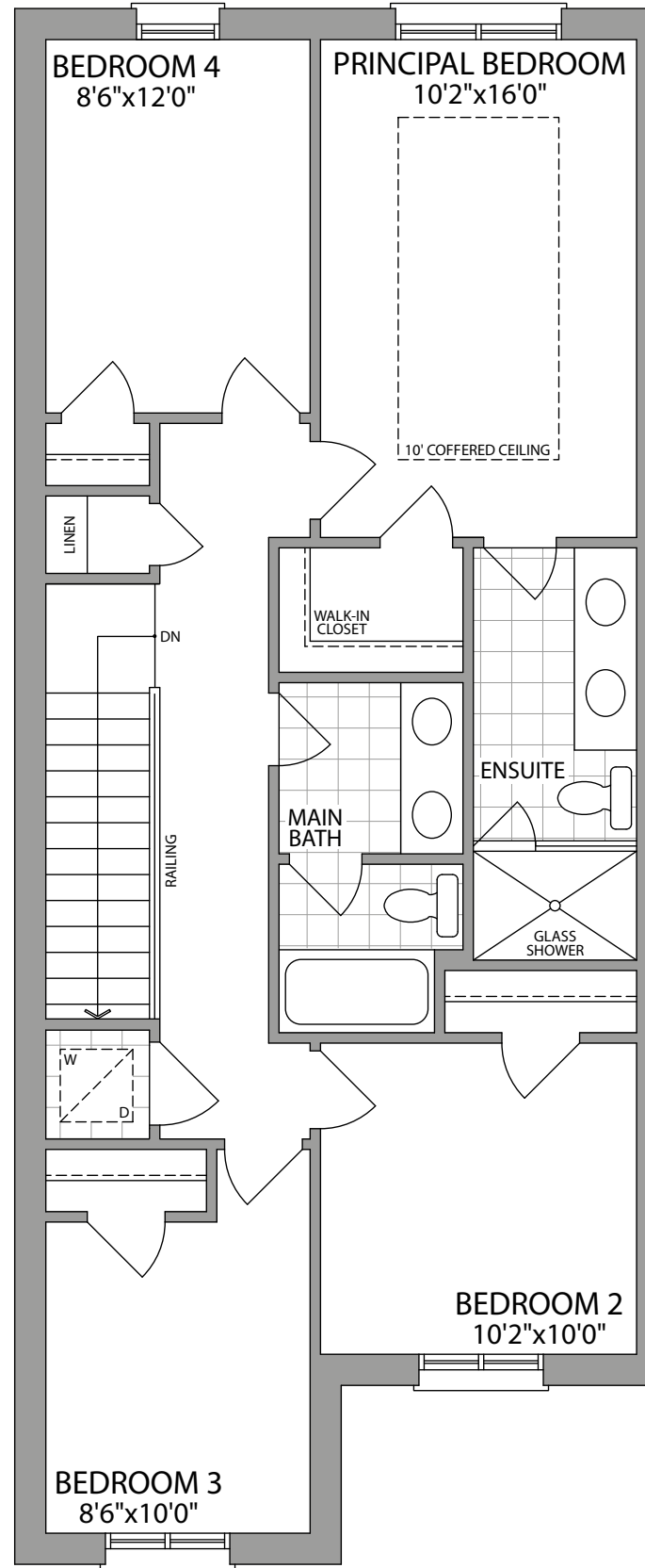
SECOND FLOOR ELEVATION 1C
