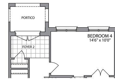
GROUND FLOOR ELEVATION 2
