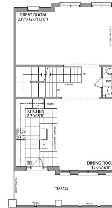
MAIN FLOOR ELEVATION 2
