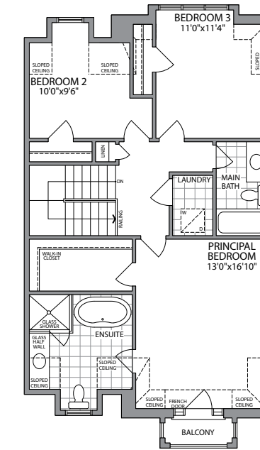
THIRD FLOOR ELEVATION 2
