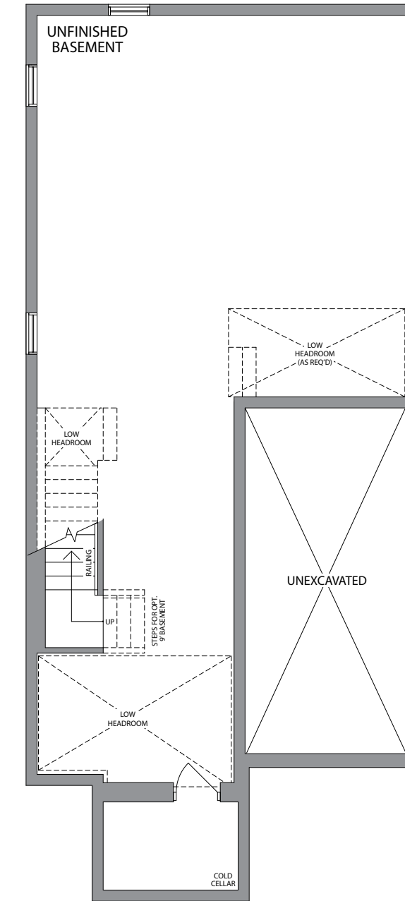
BASEMENT ELEVATION 1
