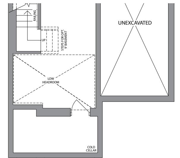
BASEMENT ELEVATION 2
