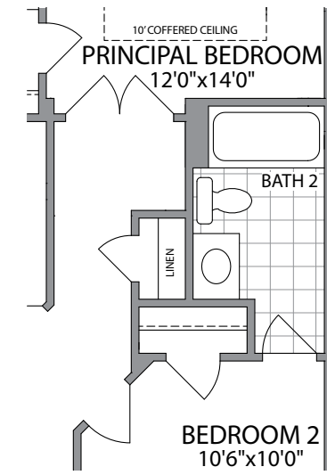
OPT. SECOND FLOOR 3 BEDROOMS W/EXTRA BATH
