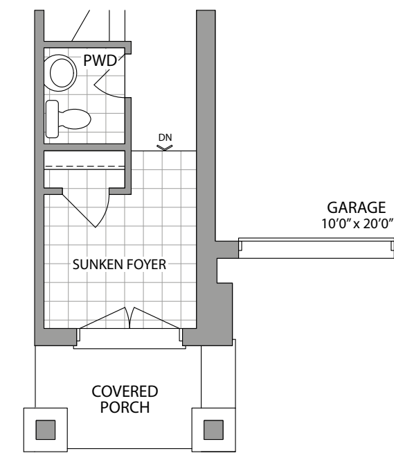
GROUND FLOOR ELEVATION 2
