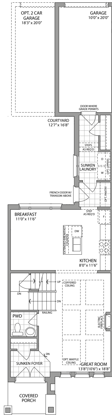
GROUND FLOOR ELEVATION 1
