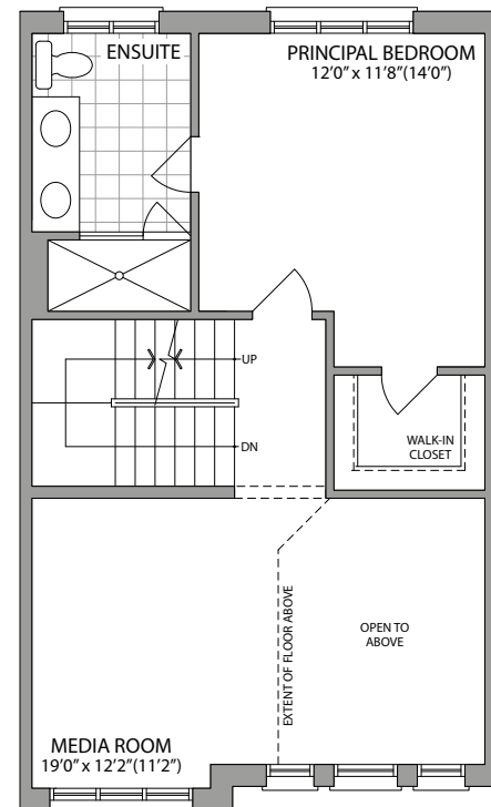
SECOND FLOOR ELEVATION 1
