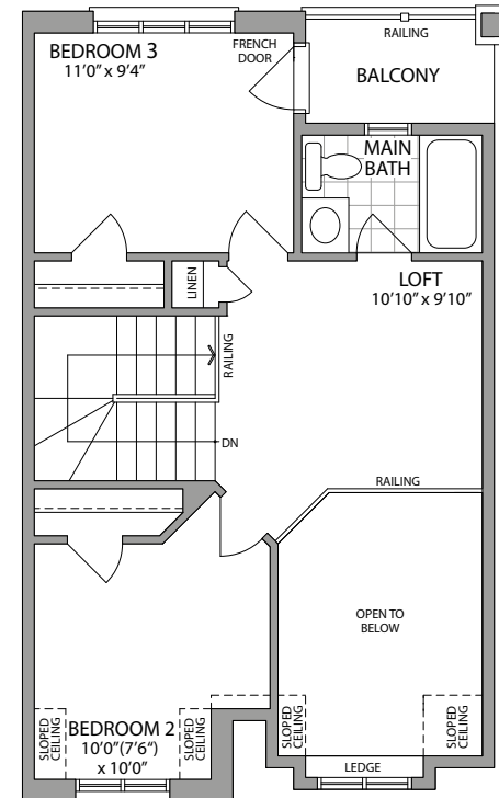
THIRD FLOOR ELEVATION 1
