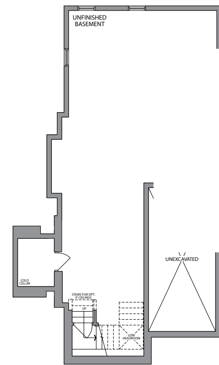
BASEMENT ELEVATION 2C
