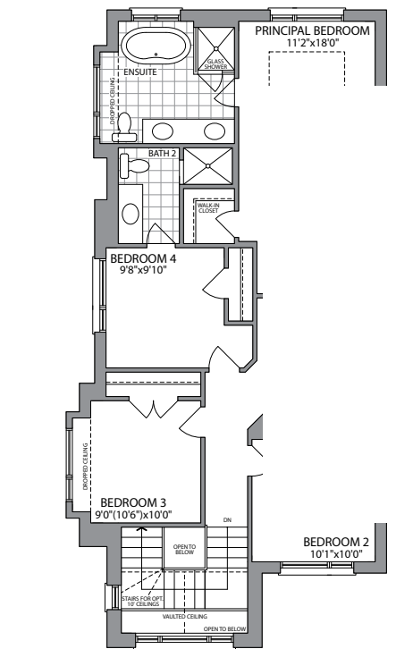
OPT. SECOND FLOOR W/EXTRA BATH ELEVATION 2C
