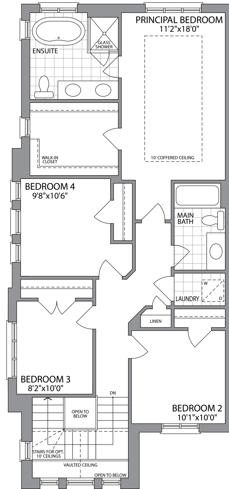
SECOND FLOOR ELEVATION 1C
