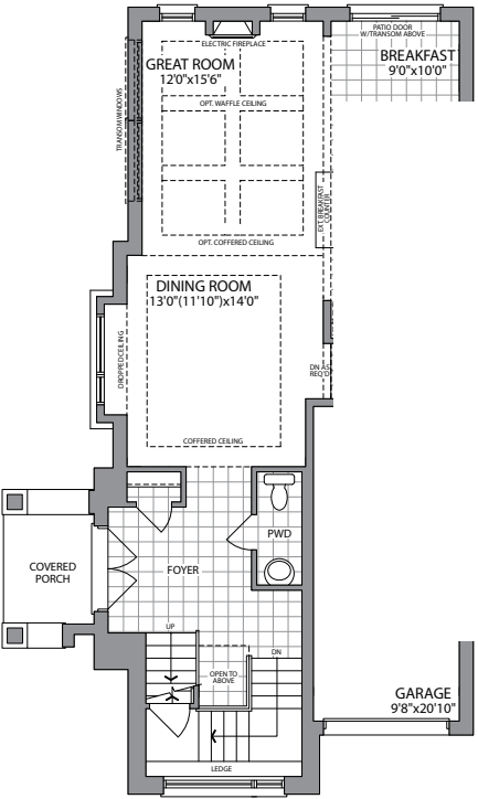
GROUND FLOOR ELEVATION 2C
