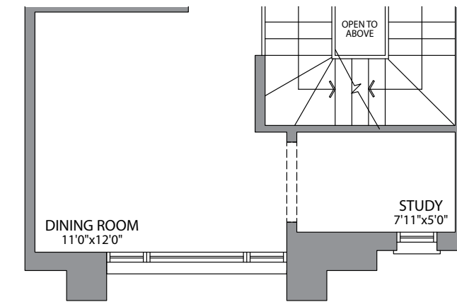
MAIN FLOOR ELEVATION 2
