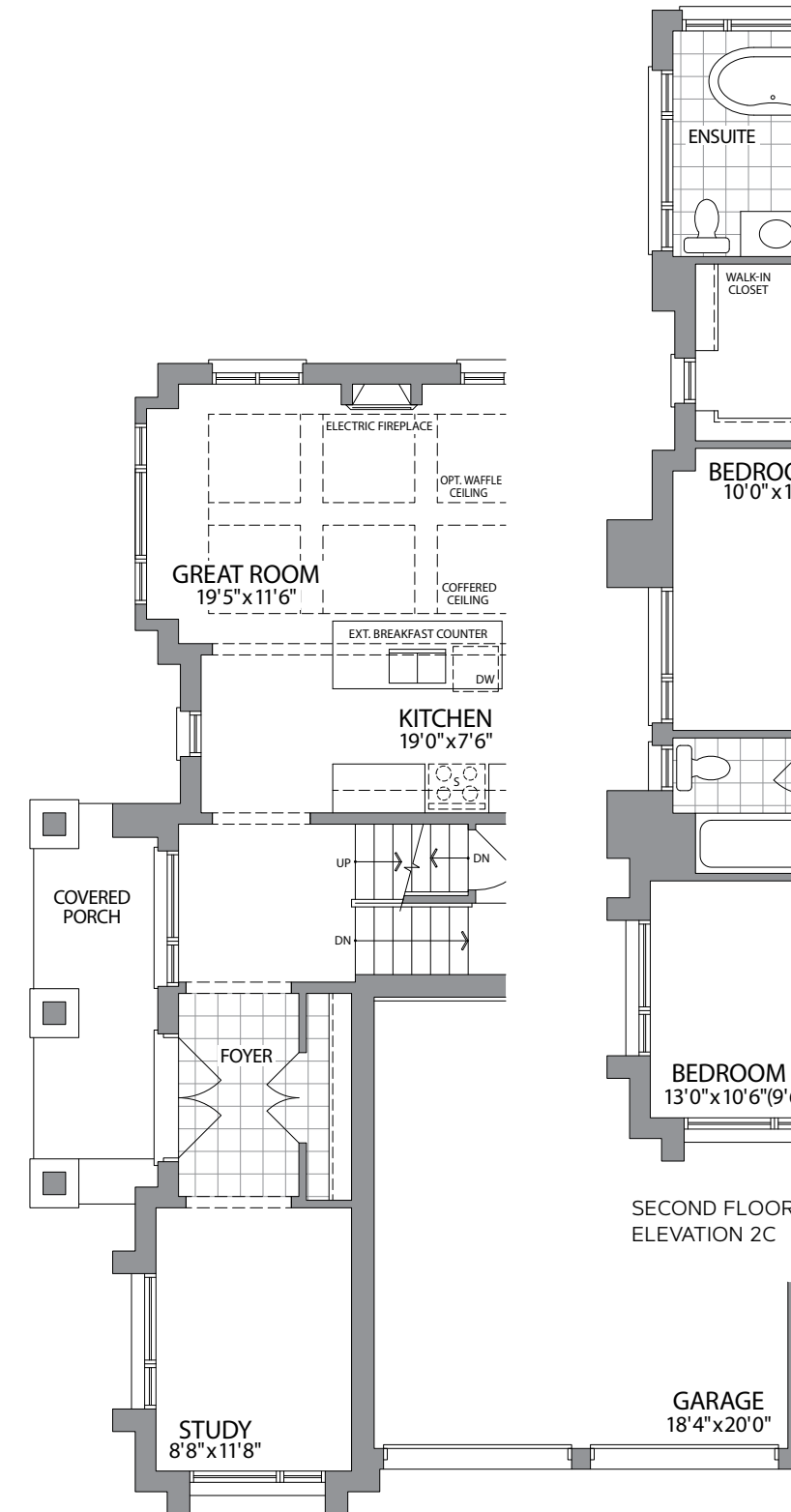
GROUND FLOOR ELEVATION 2C
