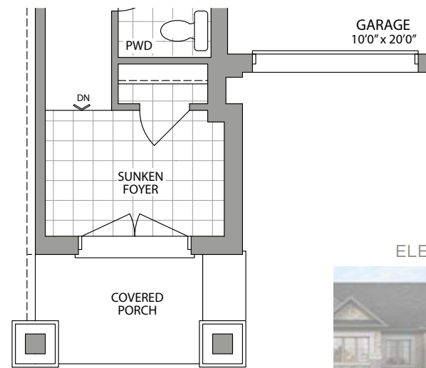
GROUND FLOOR ELEVATION 2/2C
