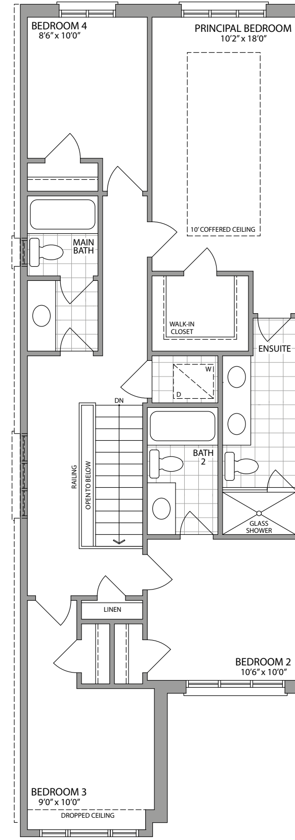
OPT. SECOND FLOOR W/4 BEDROOMS ELEVATION 1/1C
