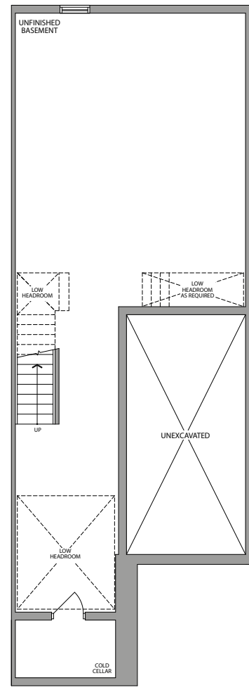
BASEMENT ELEVATION 1
