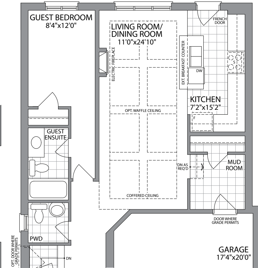
OPT. GROUND FLOOR W/GUEST BEDROOM ELEVATION 1 & 2
