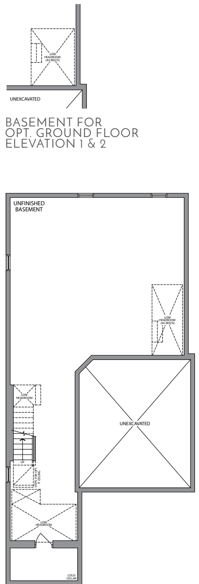
BASEMENT ELEVATION 1 & 2
